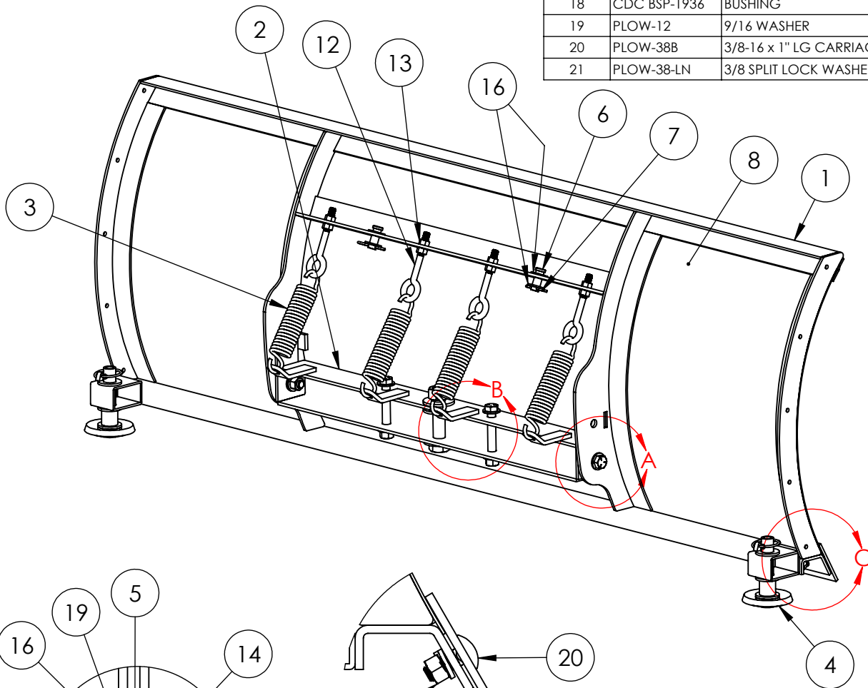
52" Plow with Standard cutting edge
